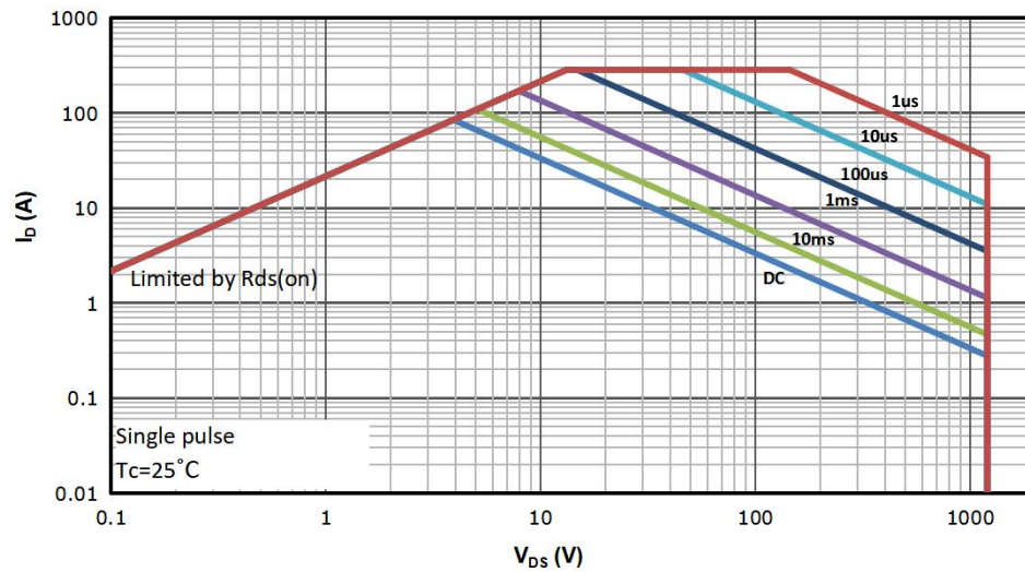
Fig 13: Safe Operating Area
